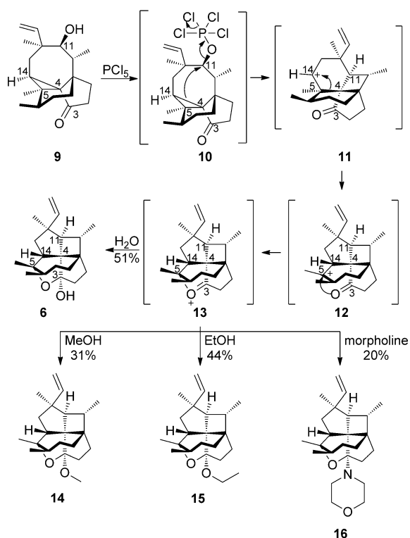
Scheme 3. Proposed mechanism for the formation of 6 : Alcohol activation and displacement affords the secondary carbocation 11 , which undergoes a 1,2-migration to form the tertiary carbocation 12 . The tertiary carbocation is trapped by the carbonyl group to form oxocarbenium 13 , which forms hemiketal 6 upon quenching with water. Quenching the reaction with methanol, ethanol, or morpholine leads to the corresponding ketal or aminal ( 14 – 16 ).
